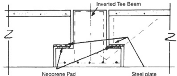
Neoprene Pad
