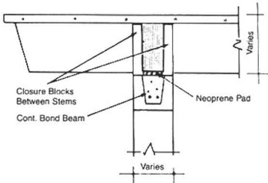
Cantilevered End-Roof
