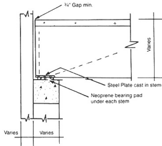
Sidewall End Bearing Detail For Floor or Roof
