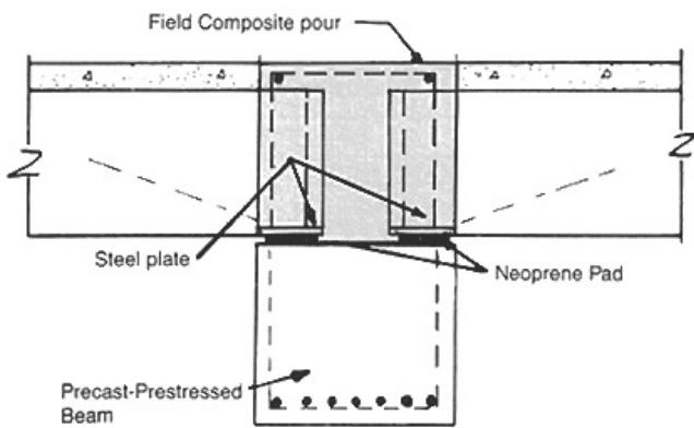
Steel plate
