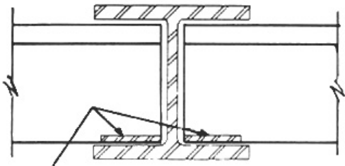
Steel plates cast in Double Tee Stem
