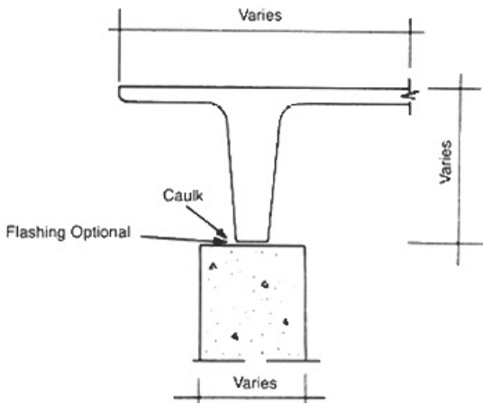
Sidewall Detail – Roof
