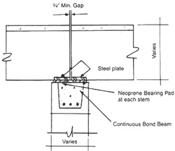
Double Tee to Interior Wall For Floor or Roof
