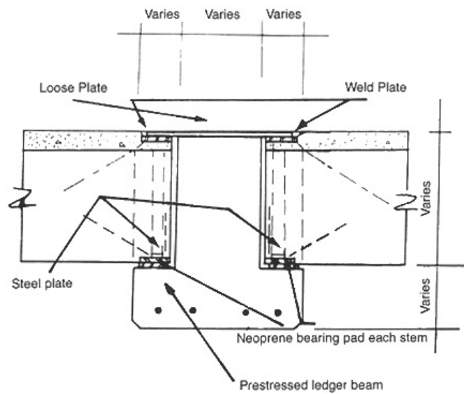
Double Tee to Interior Beam For Floor or Roof
